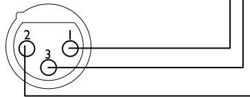
Female XLR
