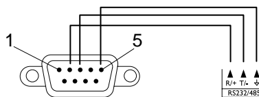
Male DB9
