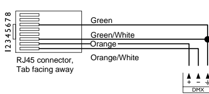
RJ45 (Philips, Traxon, Martin)
