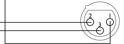
Female XLR
