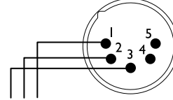
Male XLR (DMX in)
