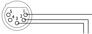
Female XLR (DMX out)
