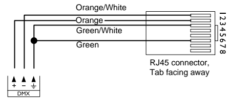
RJ45 (Philips, Traxon, Martin)
